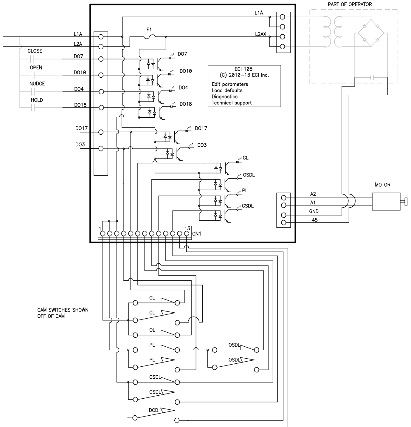
Figure 9 - 109-4 LCD Wiring diagram
