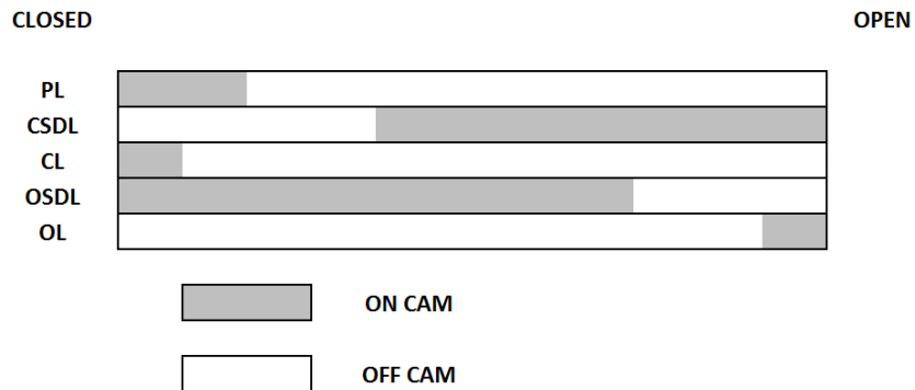
Figure 8 - CAM Profile
